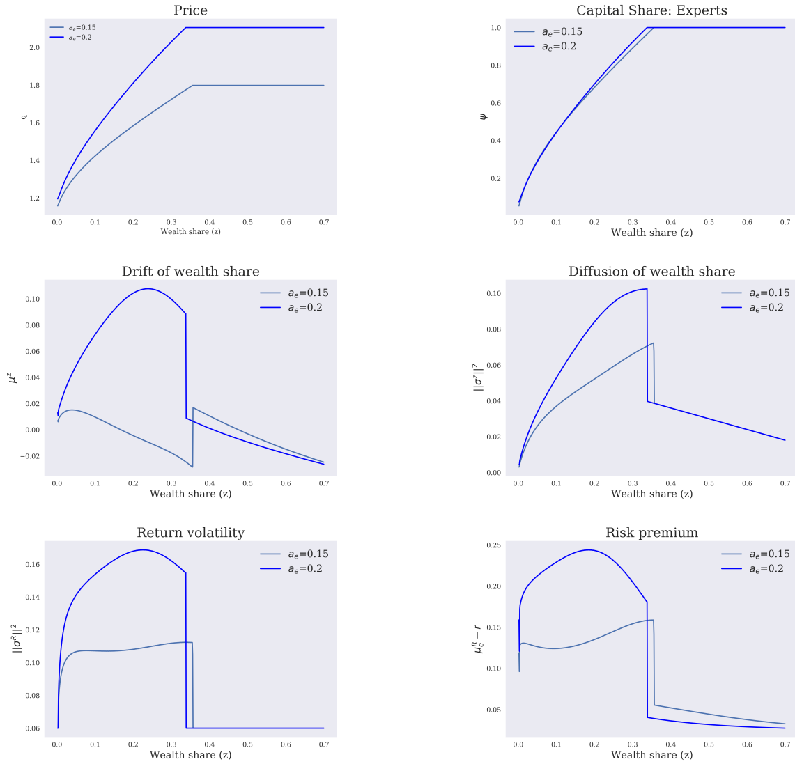
Figure 2: Model solution
